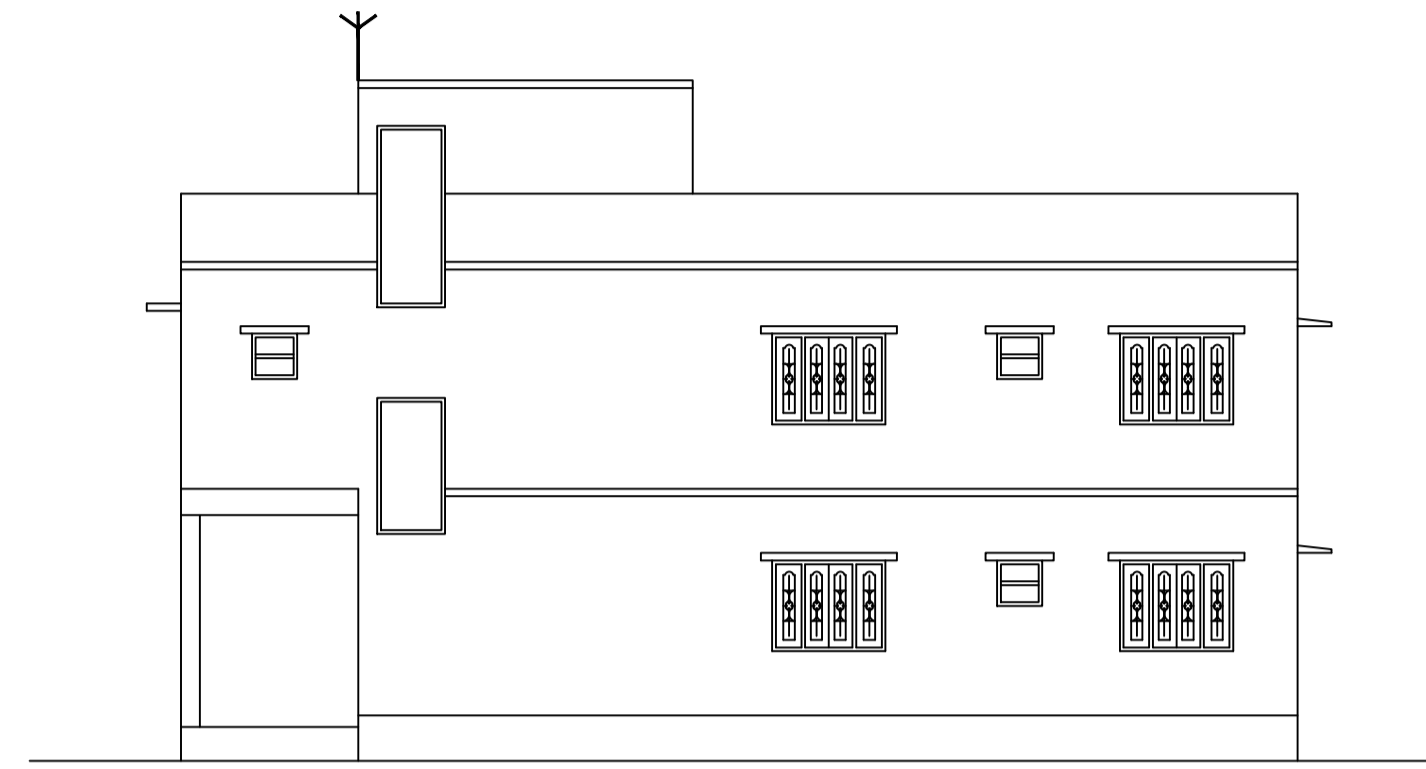
R. SIDE ELEVATION SCALE : (1:100)
