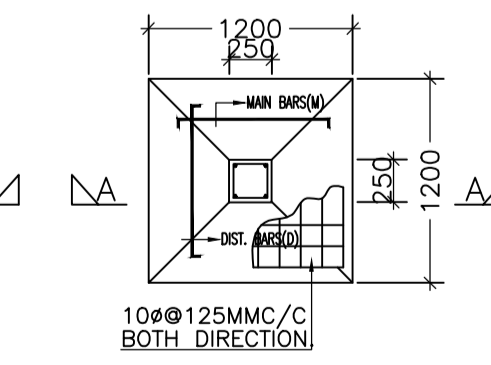
FOUNDATION PLAN OF CLOUMN
