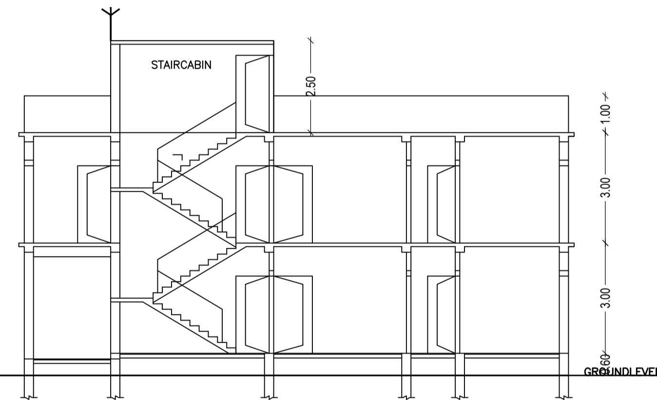
SECTION ON: <2-2> SCALE : (1:100)
