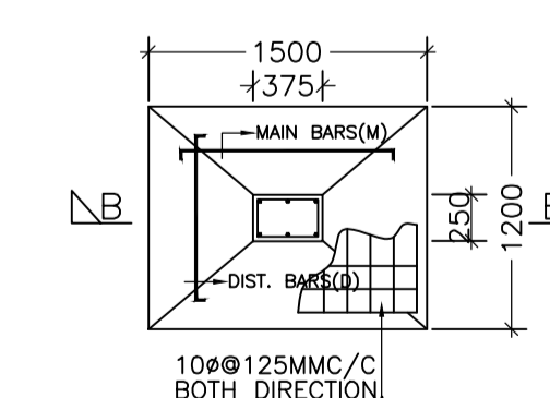
FOUNDATION PLAN OF CLOUMN
