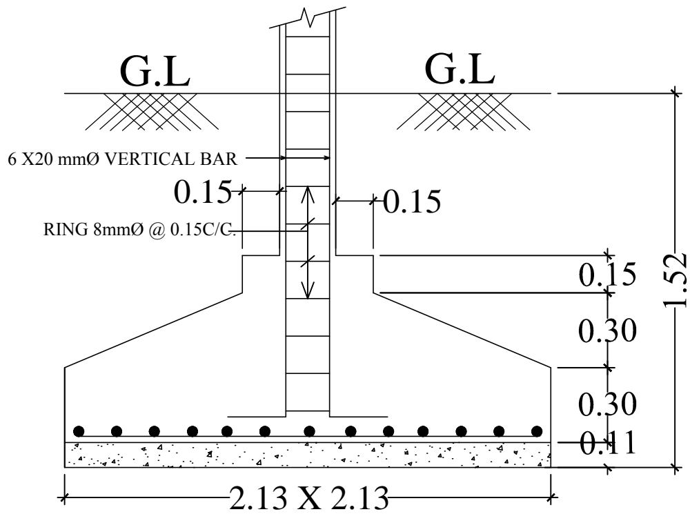
SECTION OF FOOTING
