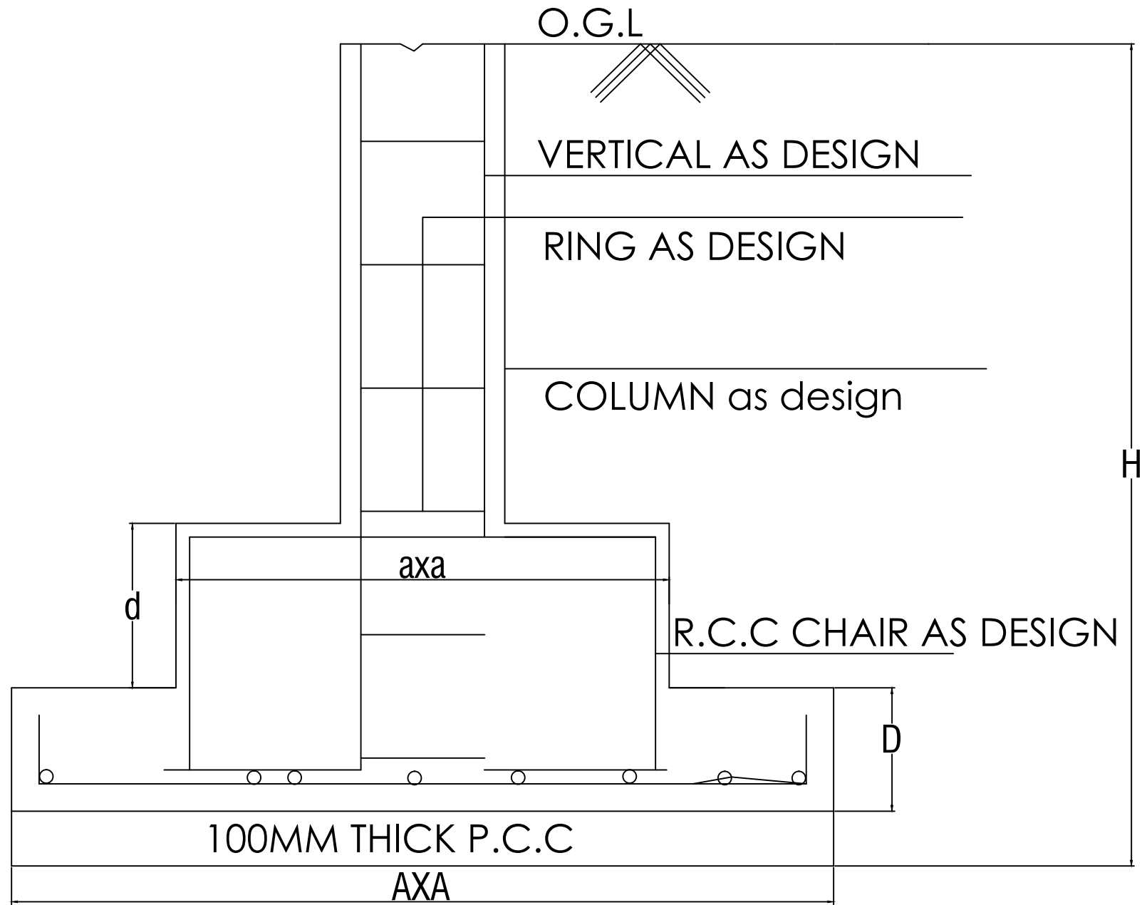
SECTION OF FOUNDATION
