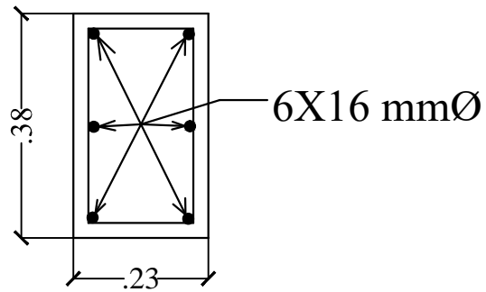
SECTION OF COLUMN. - C1
