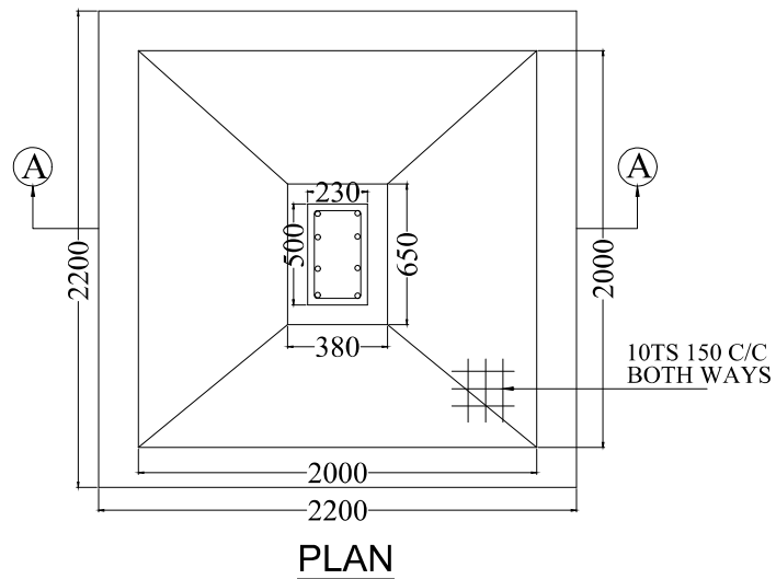
FOOTING PLAN (AS/STRL. DESIGN) SCALE N.T.S
