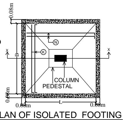
C.S. OF COLUMN . SIZE - 0.23M X 0.38M
