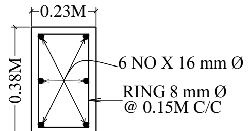
C.S. OF COLUMN . SIZE - 0.23M X 0.38M
