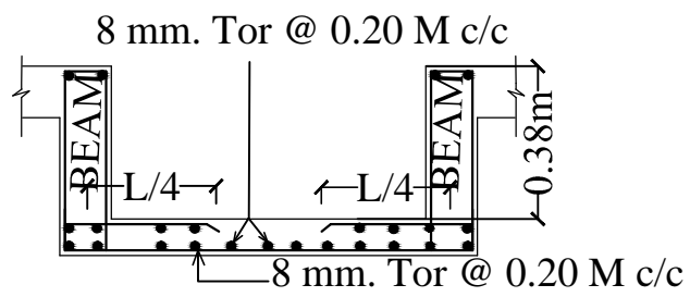
THICKNESS OF SLAB = 0.11m
