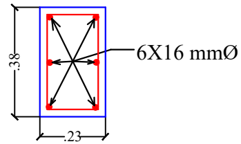
SECTION OF COLUMN. - C1
