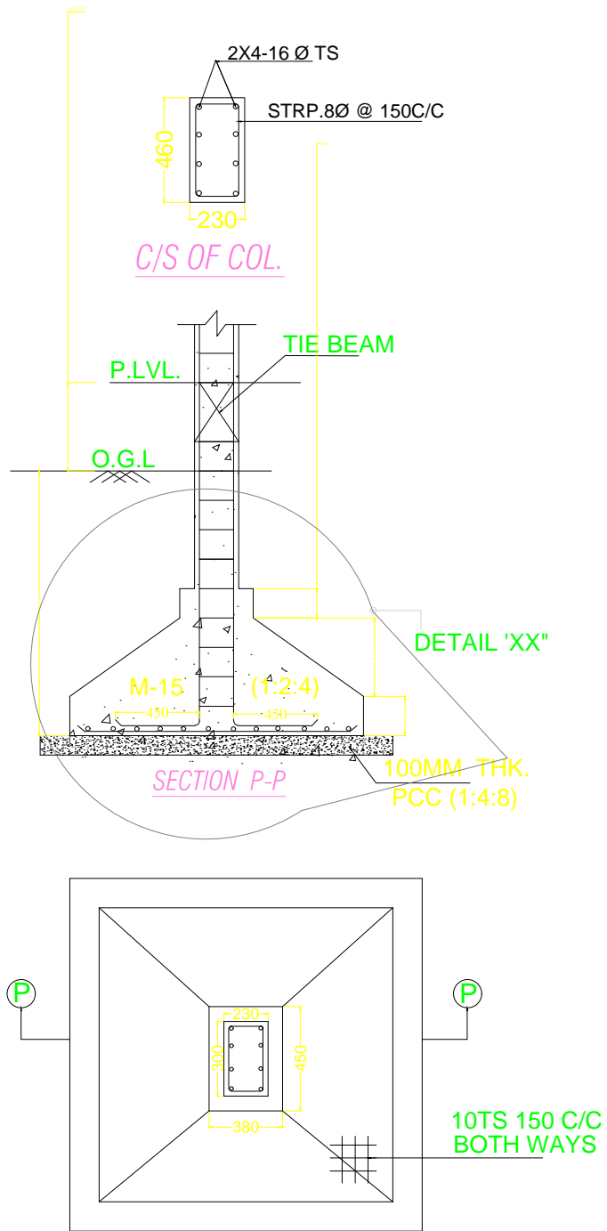
PLAN FOOTING PLAN (AS/STRL. DESIGN) SCALE N.T.S
