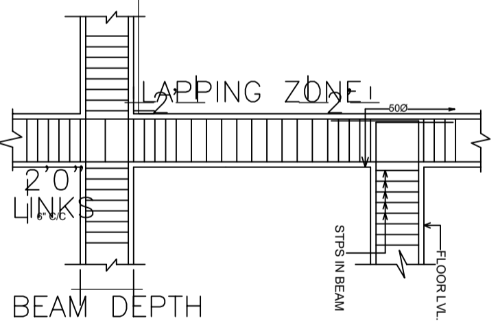
TYPICAL CROSS SECTION OF COLUMN
