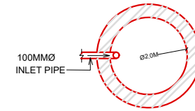
PLAN OF SOAK PIT
