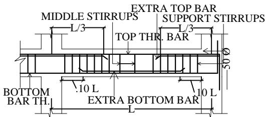
SECTION OF TYPICAL FLOOR BEAM
