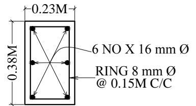
C.S. OF COLUMN SIZE - 0.23M X 0.38M
