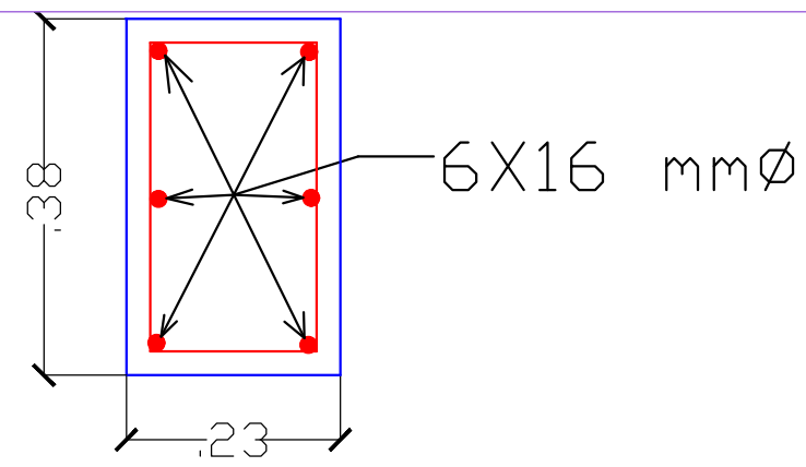
SECTION OF COLUMN, - C1
