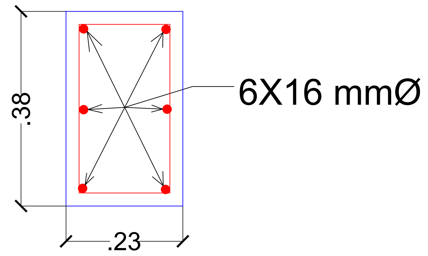
SECTION OF COLUMN. - C1
