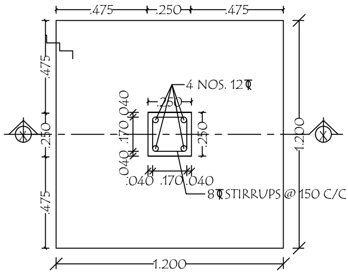
DETAILS OF COLUMN FOUNDATION
