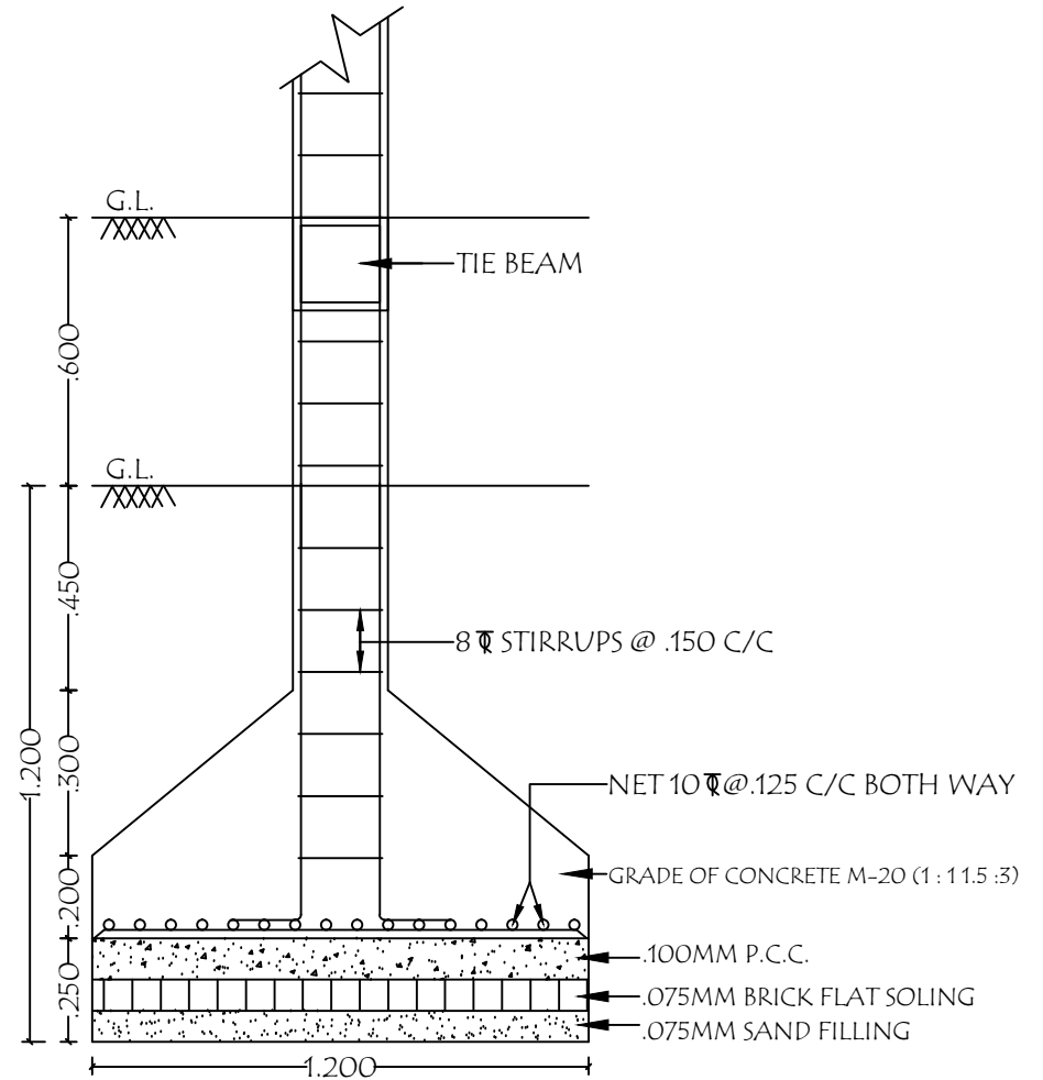
SECTION X X
