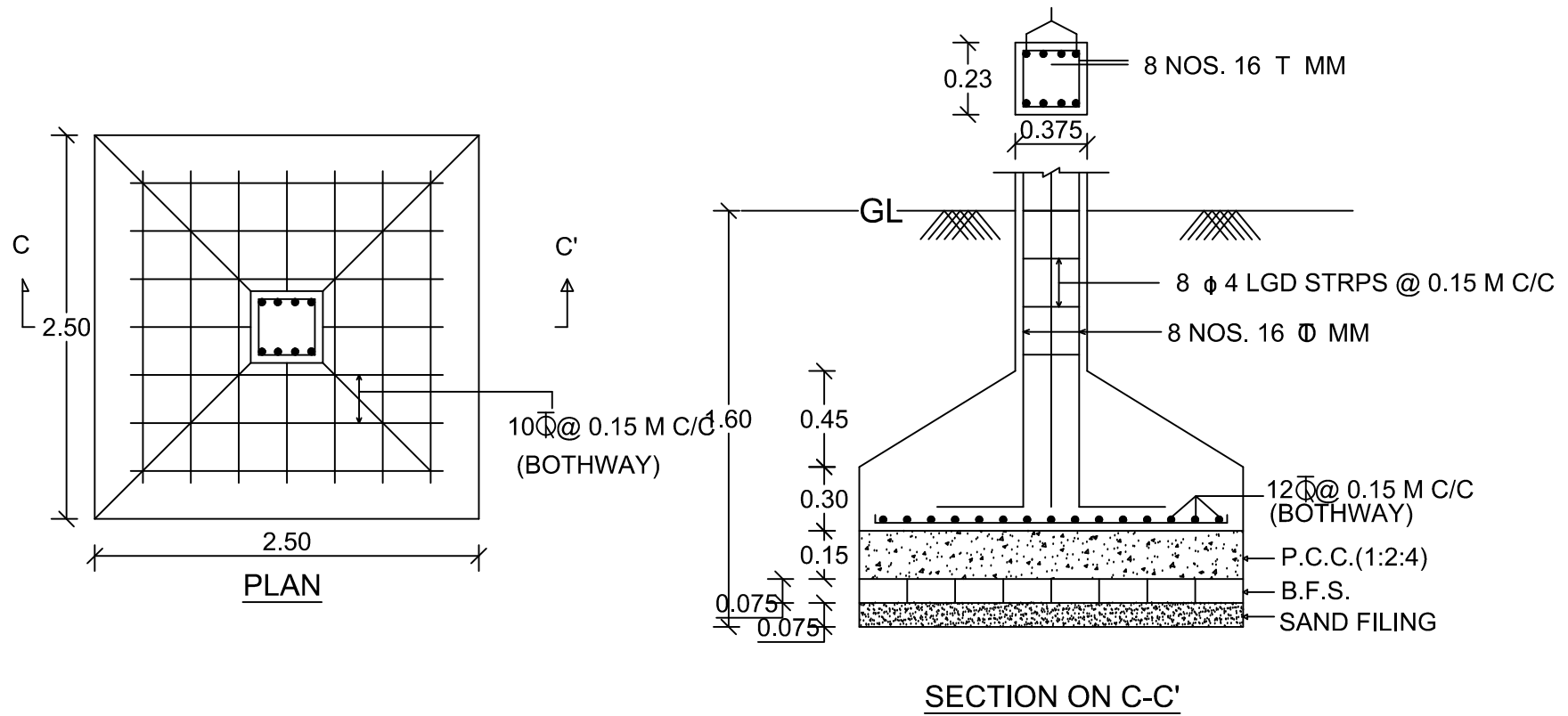
DETAILS OF FOUNDATION
