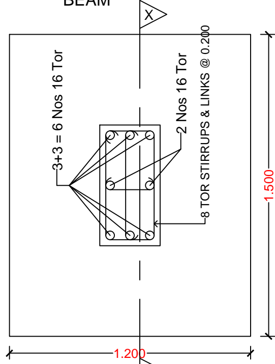
CROSS SECTION BEAM
