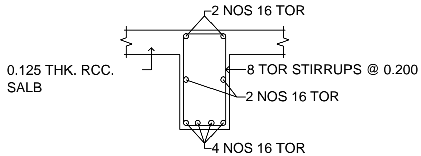
CROSS SECTION BEAM
