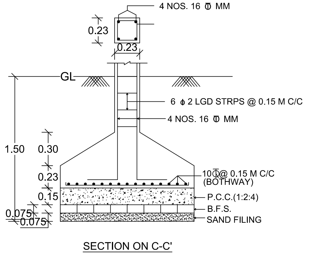
DETAILS OF COLUMN FOUNDATION
