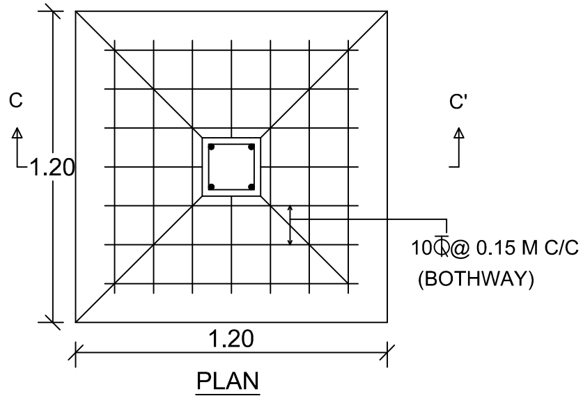
DETAILS OF COLUMN FOUNDATION
