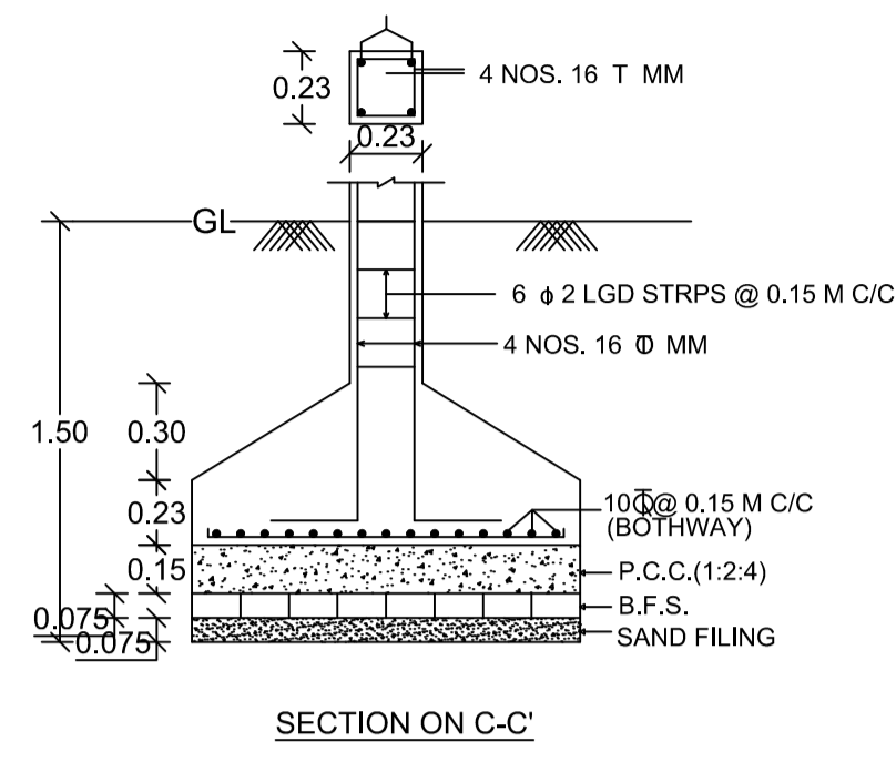
DETAILS OF FOUNDATION
