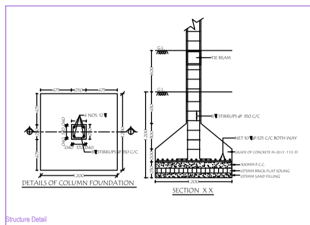
Structure Detail
