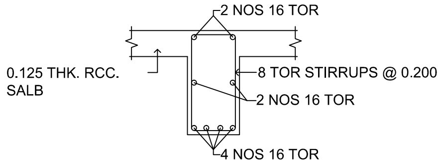
CROSS SECTION BEAM
