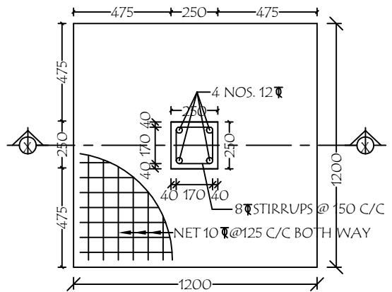
DETAILS OF COLUMN FOUNDATION Scale - N.T.S.
