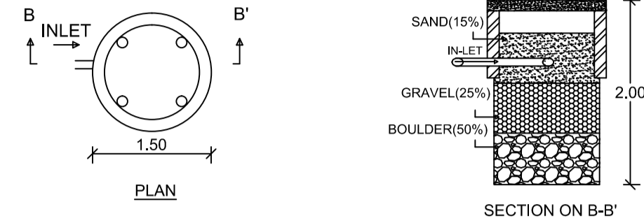
DETAILS OF WATER HARVESTING
