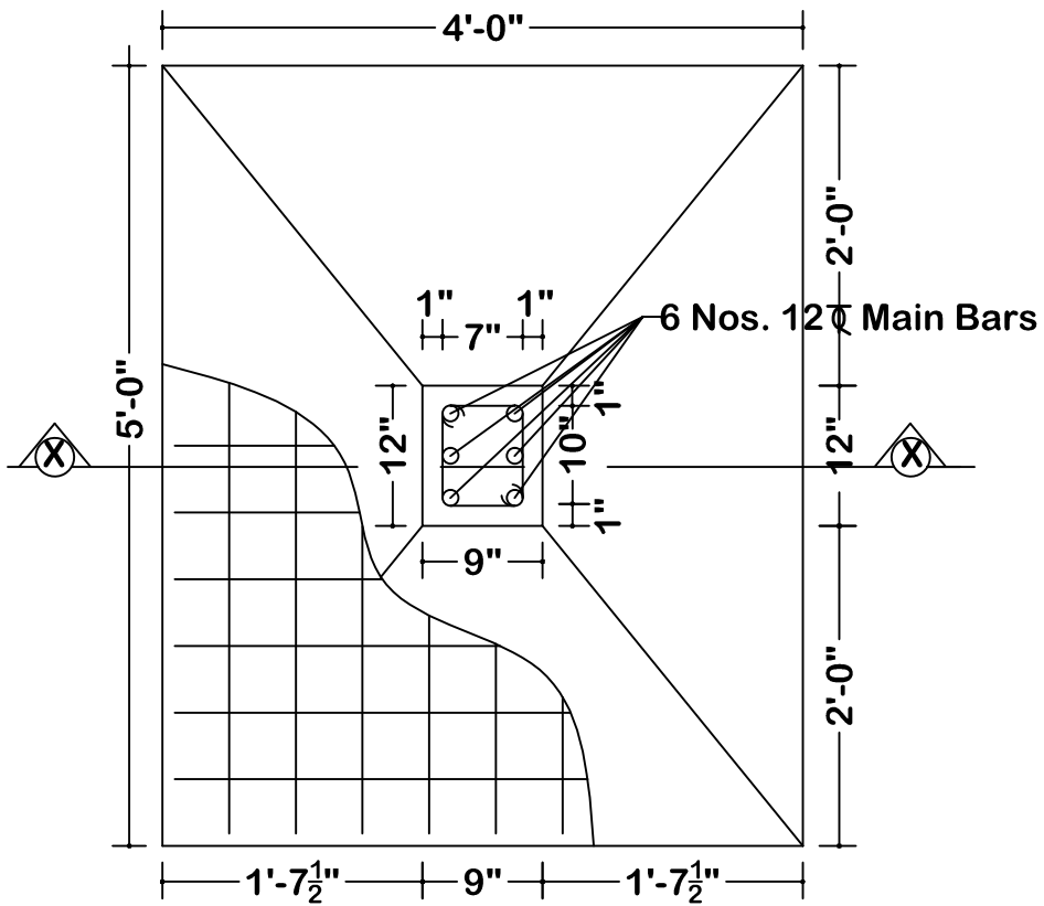
PLAN OF COLUMN FOUNDATION
