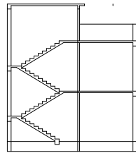
SECTION AT - AA
