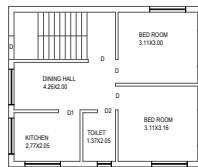
FIRST FLOOR PLAN
