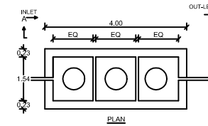
DETAILS OF SEPTIC TANK
