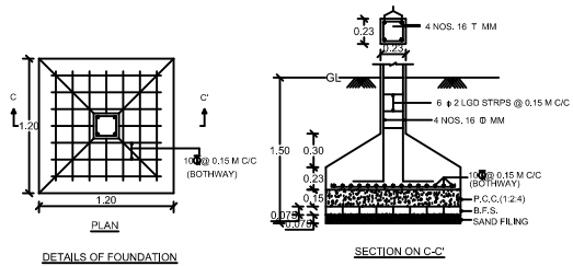
DETAILS OF FOUNDATION
