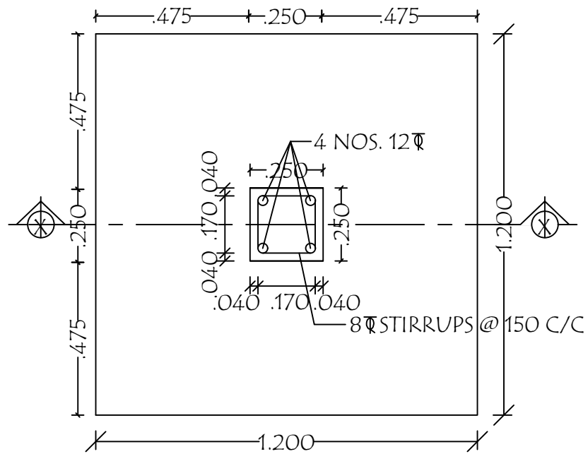
DETAILS OF COLUMN FOUNDATION
