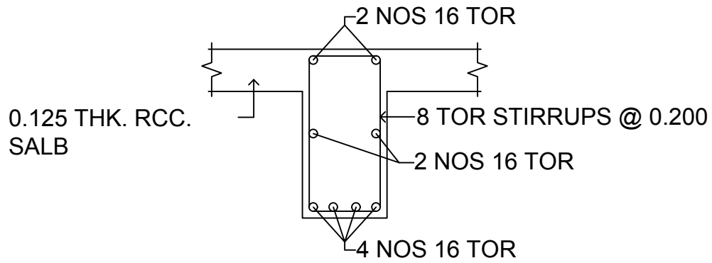
CROSS SECTION BEAM
