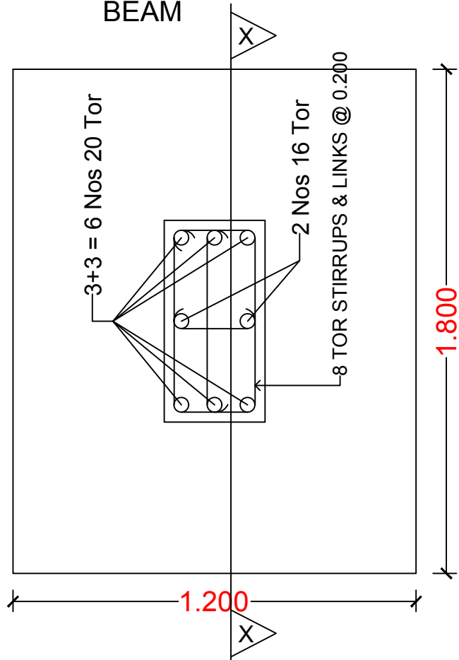
COLUMN FOUNDATION PLAN
