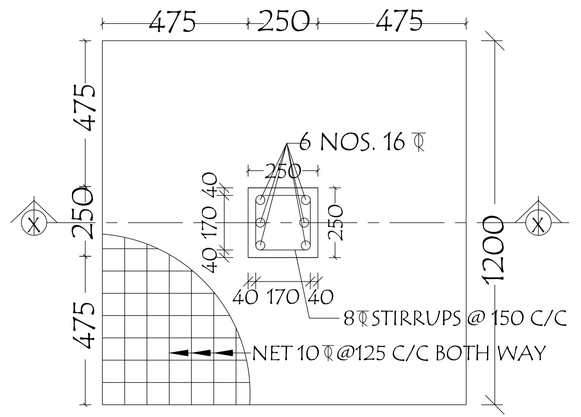
DETAILS OF COLUMN FOUNDATION SCALE = N.T.S.
