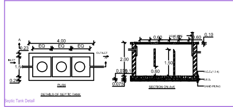
Septic Tank Detail
