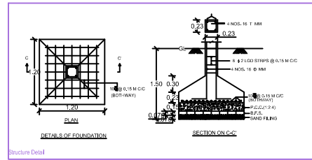
Structure Detail
