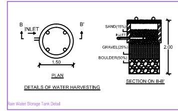
Rain Water Storage Tank Detail
