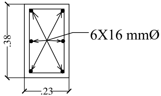
SECTION OF COLUMN. - C1
