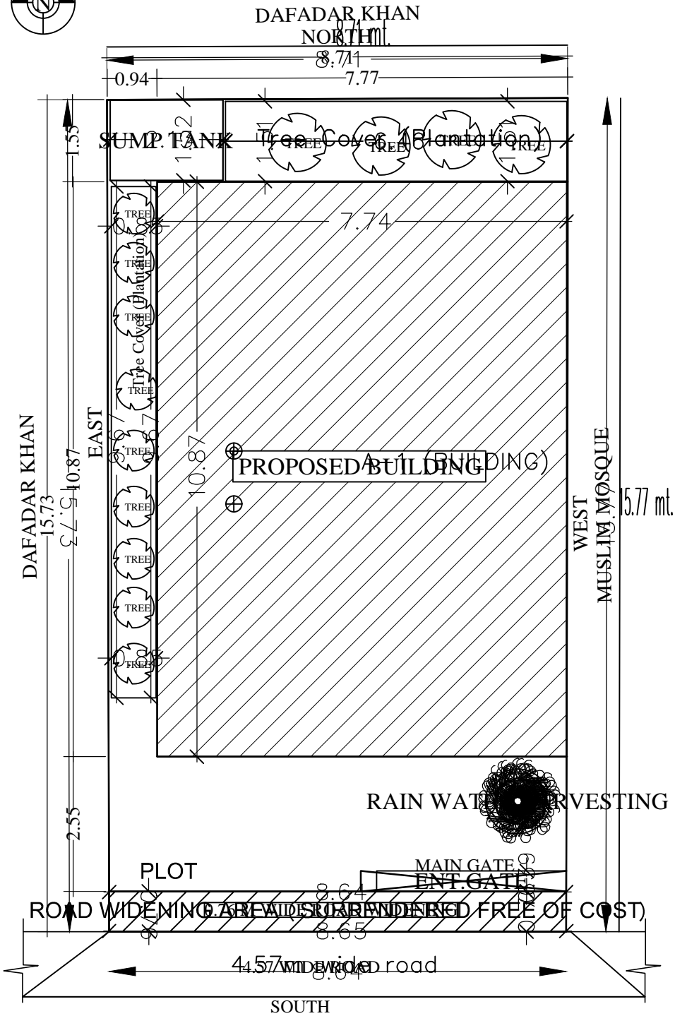
GROUND FLOOR PLAN SHOWING DRAINAGE SCALE 1:100
