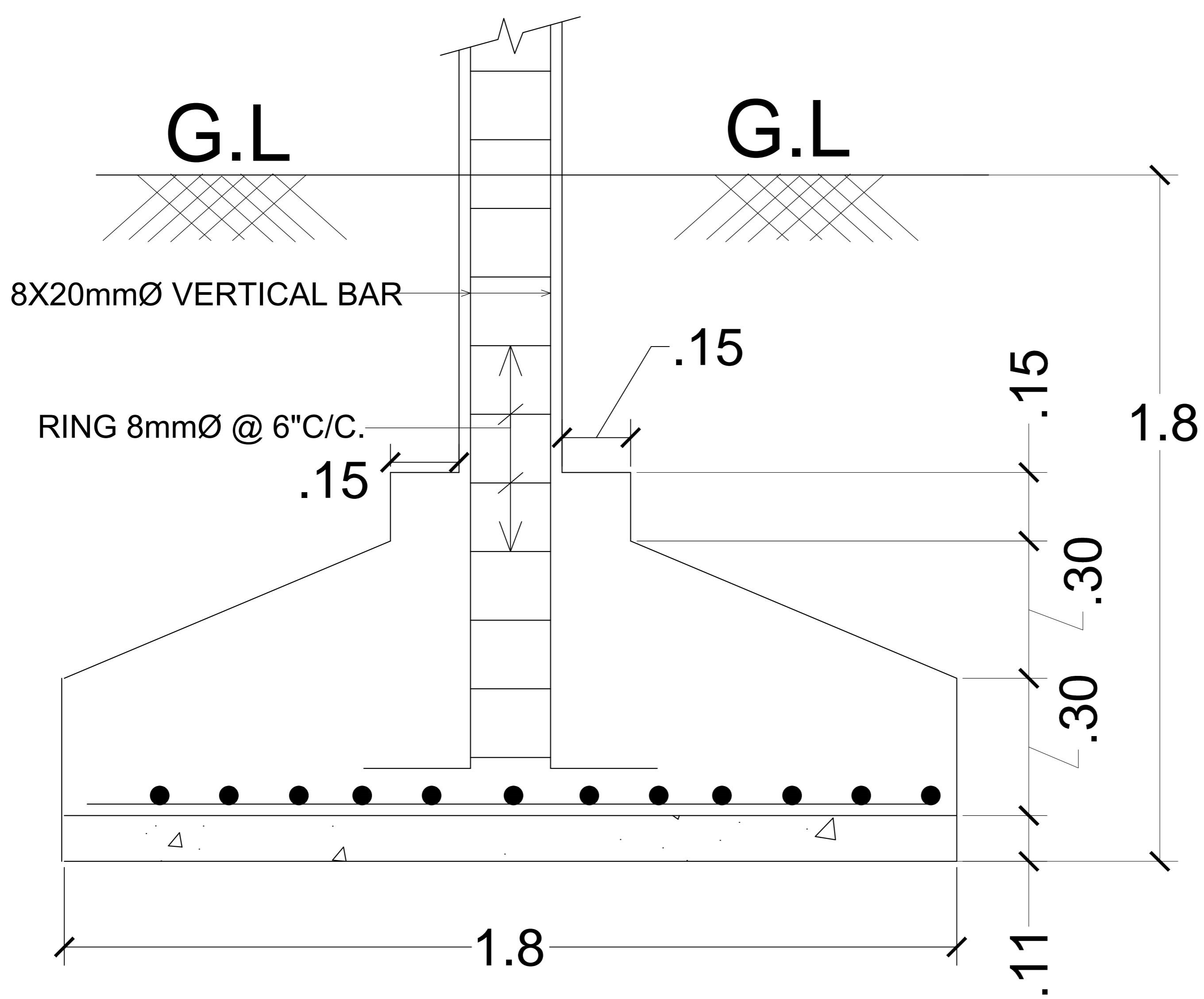
SECTION OF FOOTING
