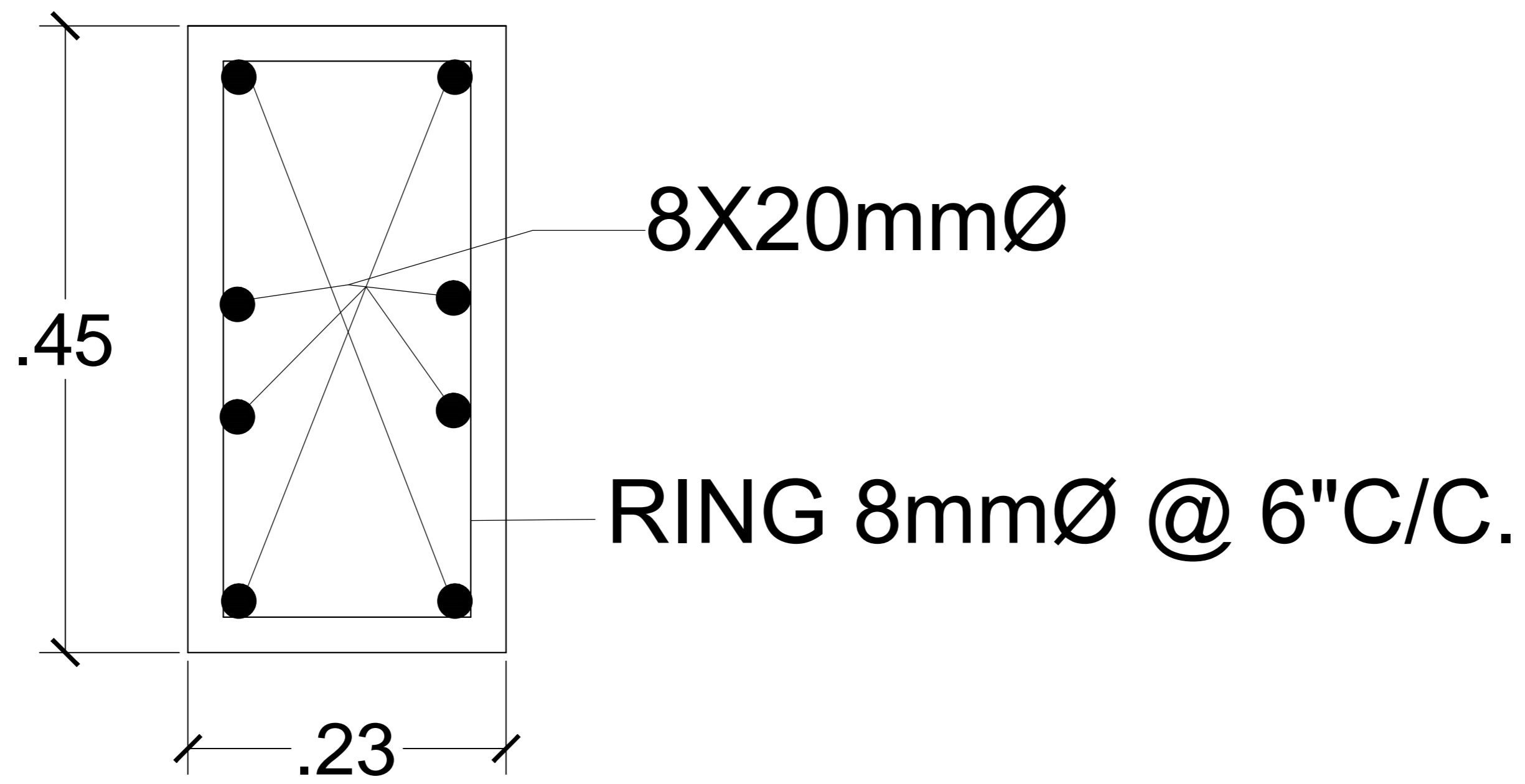
PLAN OF COLUMN.
