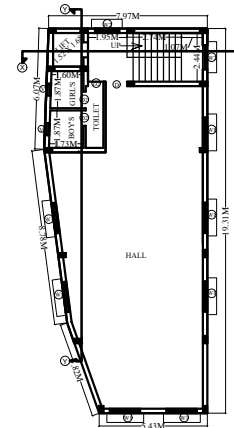
(TYPICAL) 1st, 2nd & 4th FLOOR PLAN SCALE - 1:100
