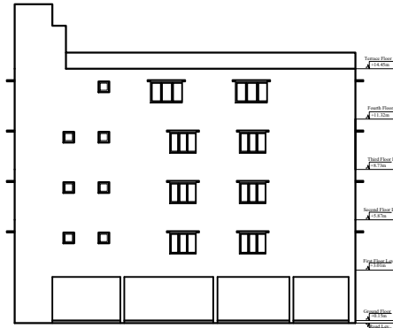
EAST SIDE ELEVATION SCALE - 1:100
