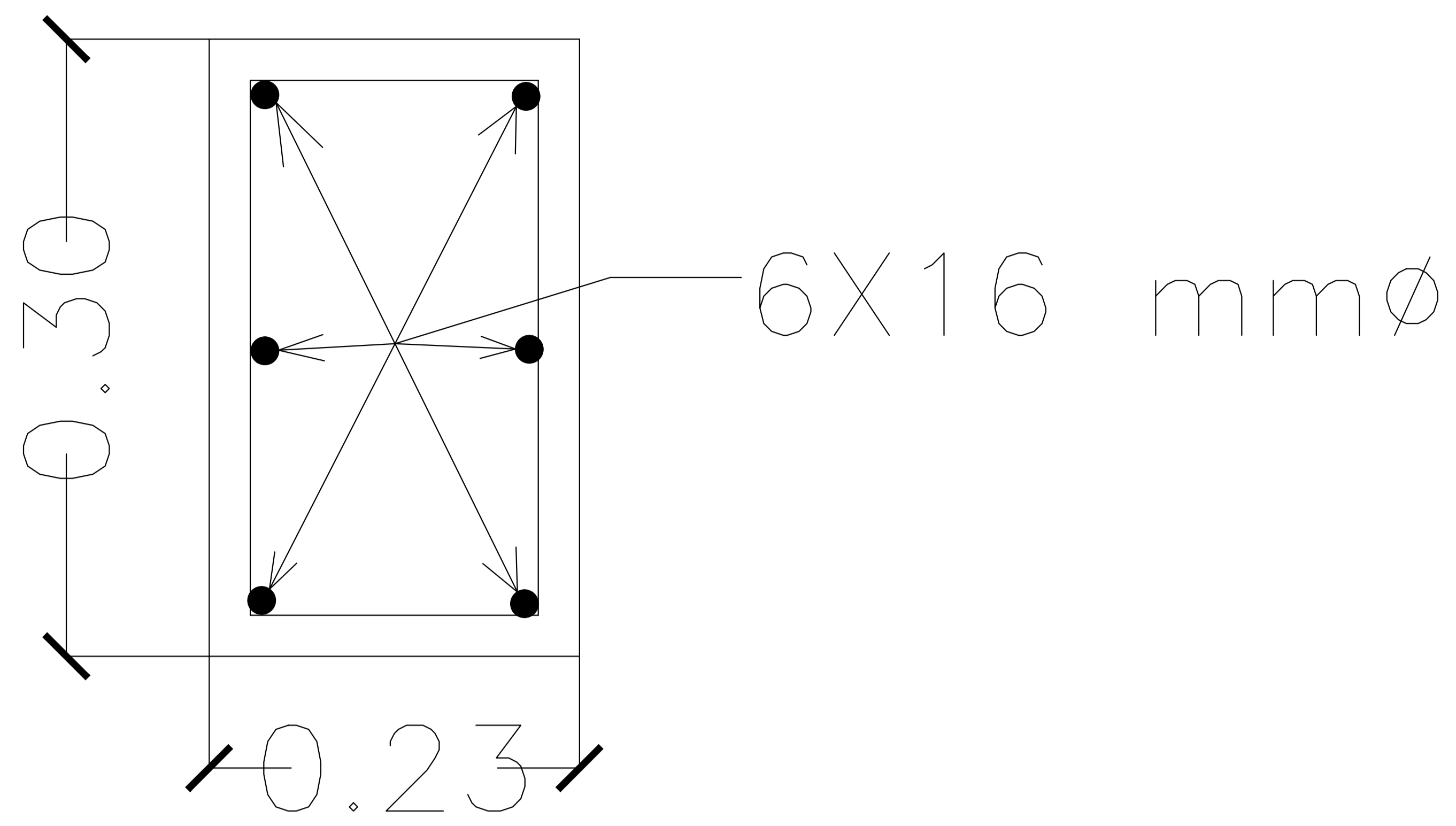
SECTION OF COLUMN
