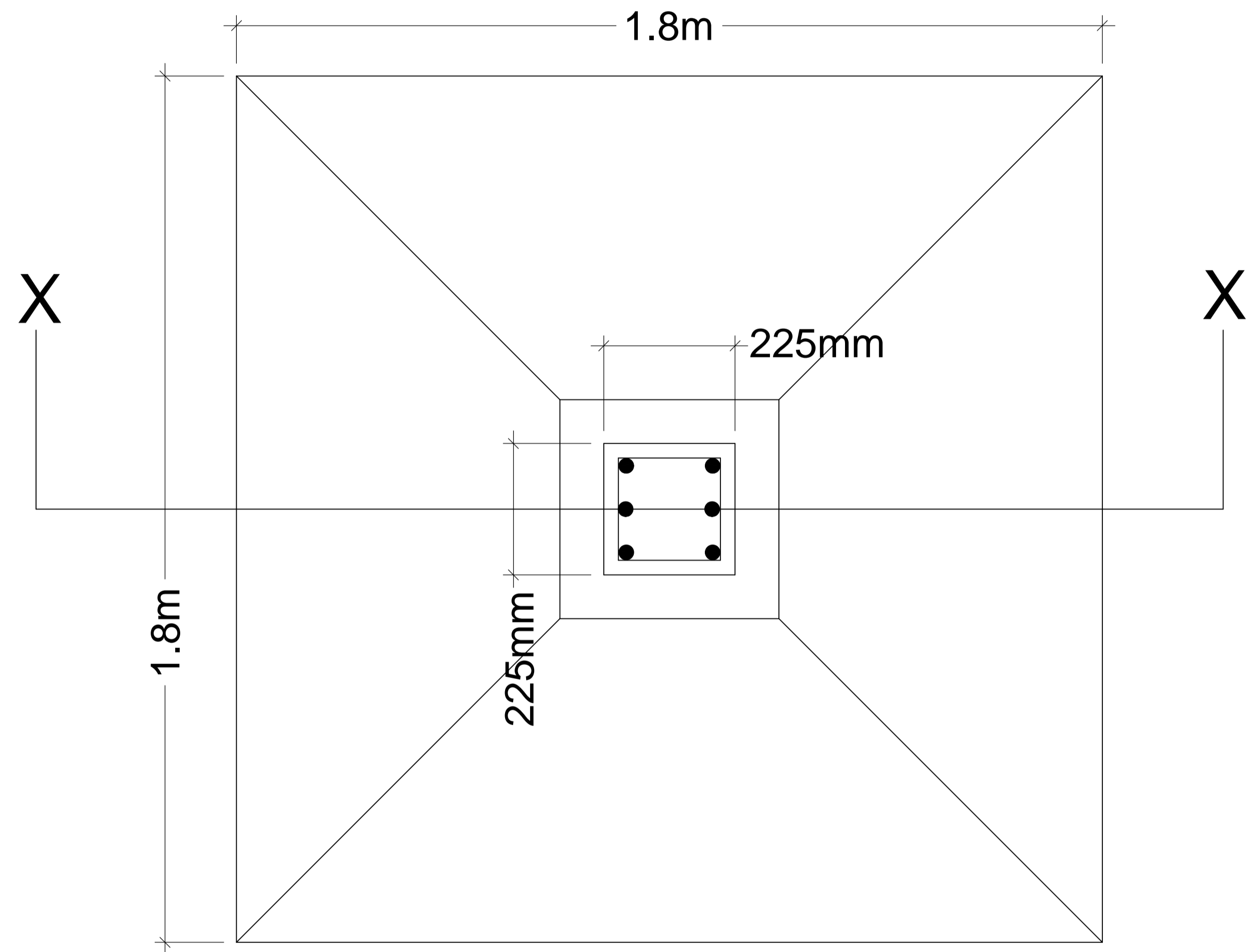
DETAIL OF FOOTING (Not to Scale)
