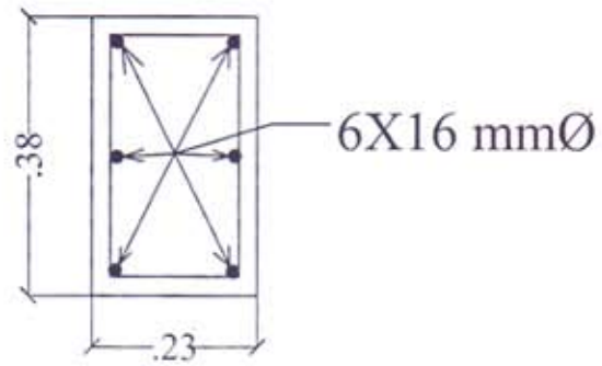
SECTION OF COLUMN. - C1
