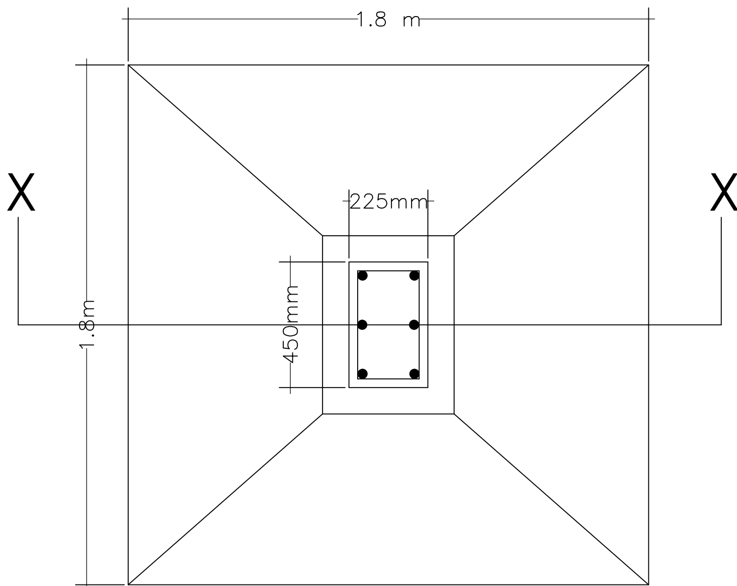
DETAIL OF FOOTING
