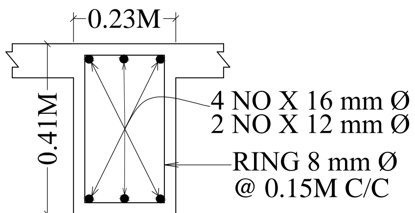
C.S. OF ROOF BEAM SIZE - 0.23M X 0.41M
