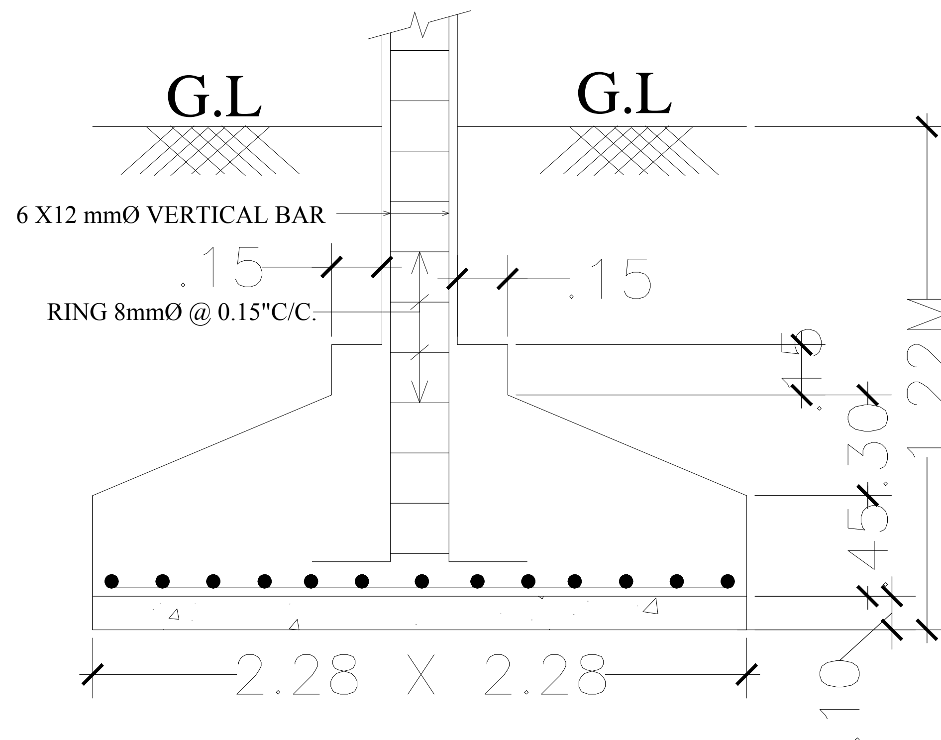
SECTION OF FOOTING
