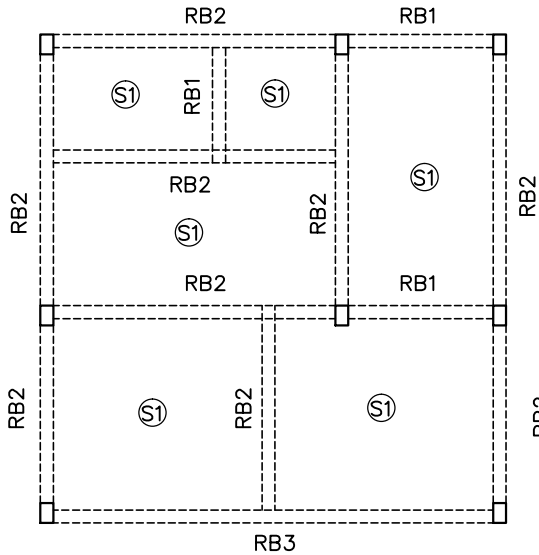
ROOF BEAM & SLAB LAYOUT
