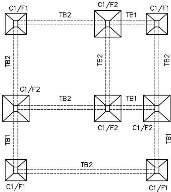
COLUMN & FOOTING & TIE-BEAM LAYOUT
