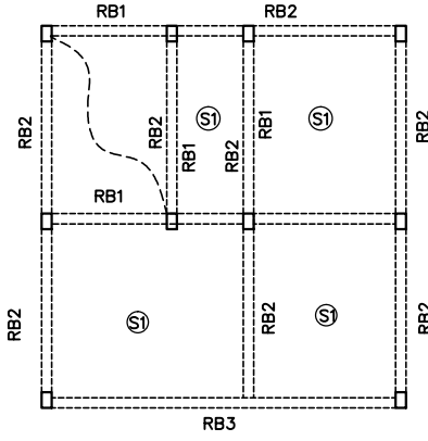
2ND ROOF BEAM & SLAB LAYOUT
