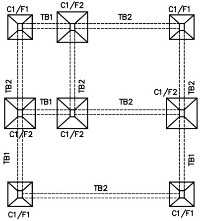
COLUMN & FOOTING & TIE-BEAM LAYOUT
