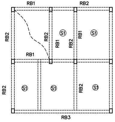
1ST ROOF BEAM & SLAB LAYOUT
