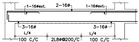
TB2(0.23x0.3)
