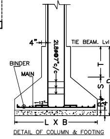
DETAIL OF COLUMN & FOOTING
