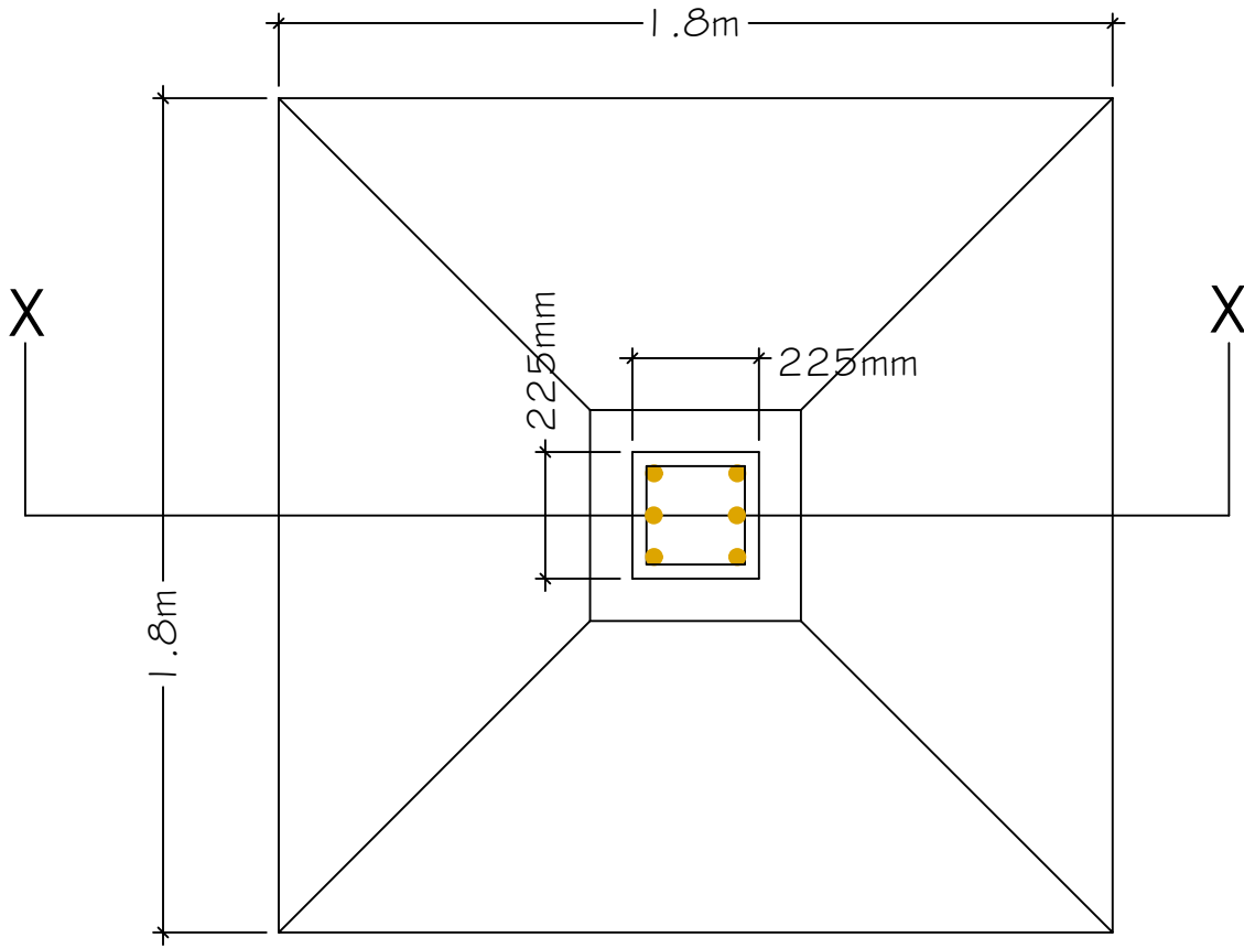
DETAIL OF FOOTING (Not to Scale)
