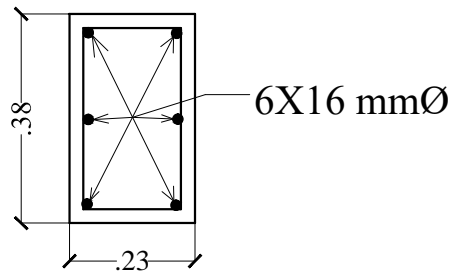
SECTION OF COLUMN. - C1
