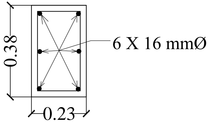
SECTION OF COLUMN.
