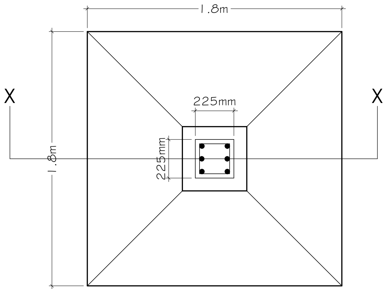
DETAIL OF FOOTING Not to Scale
