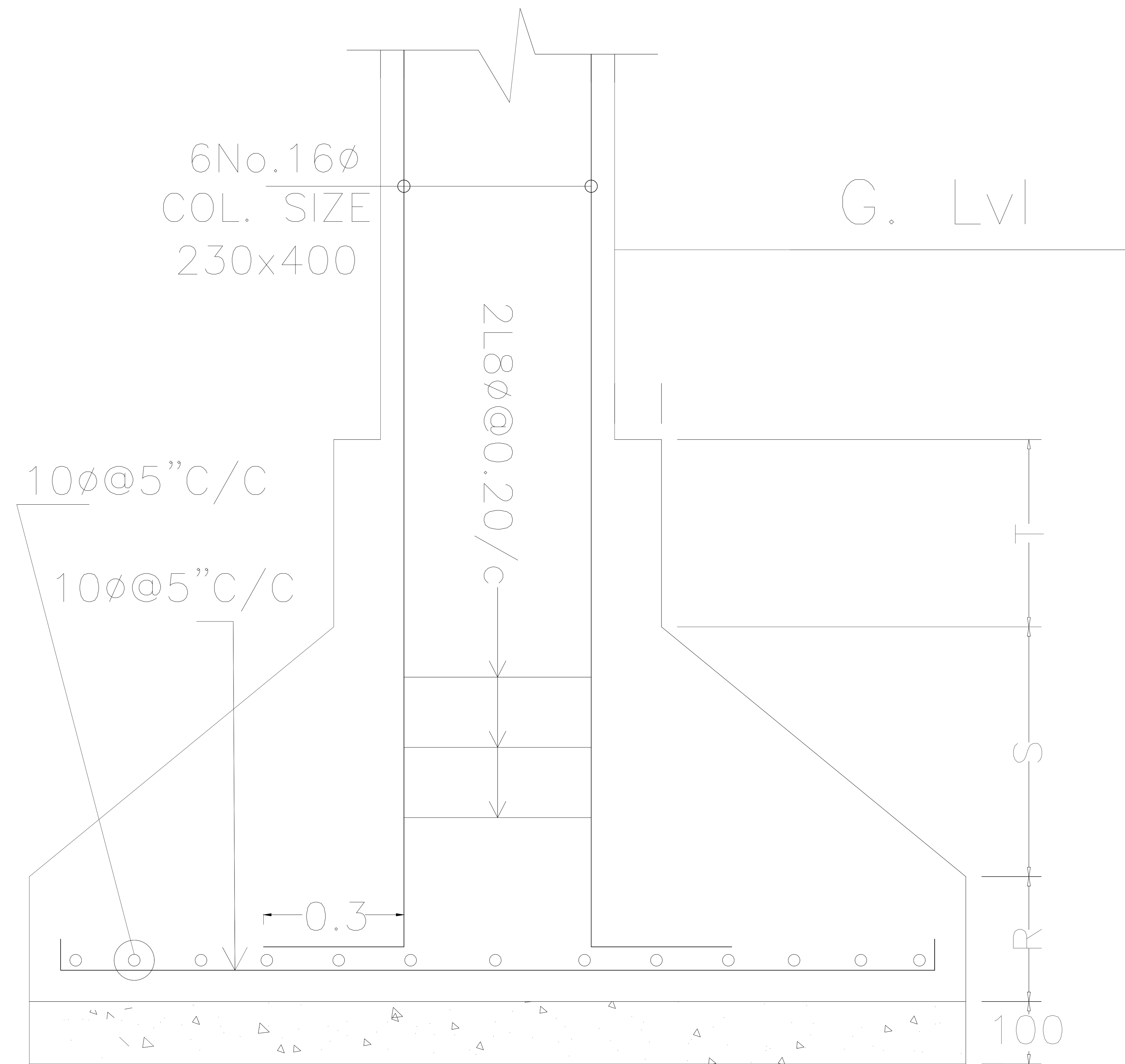
DETAIL OF COLUMN & FOOTING
