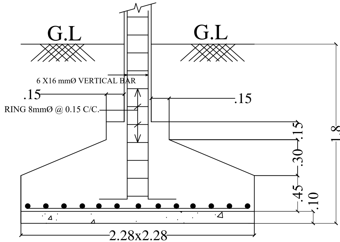
SECTION OF FOOTING
