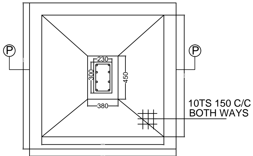
PLAN FOOTING PLAN (AS/STRL. DESIGN) SCALE N.T.S
