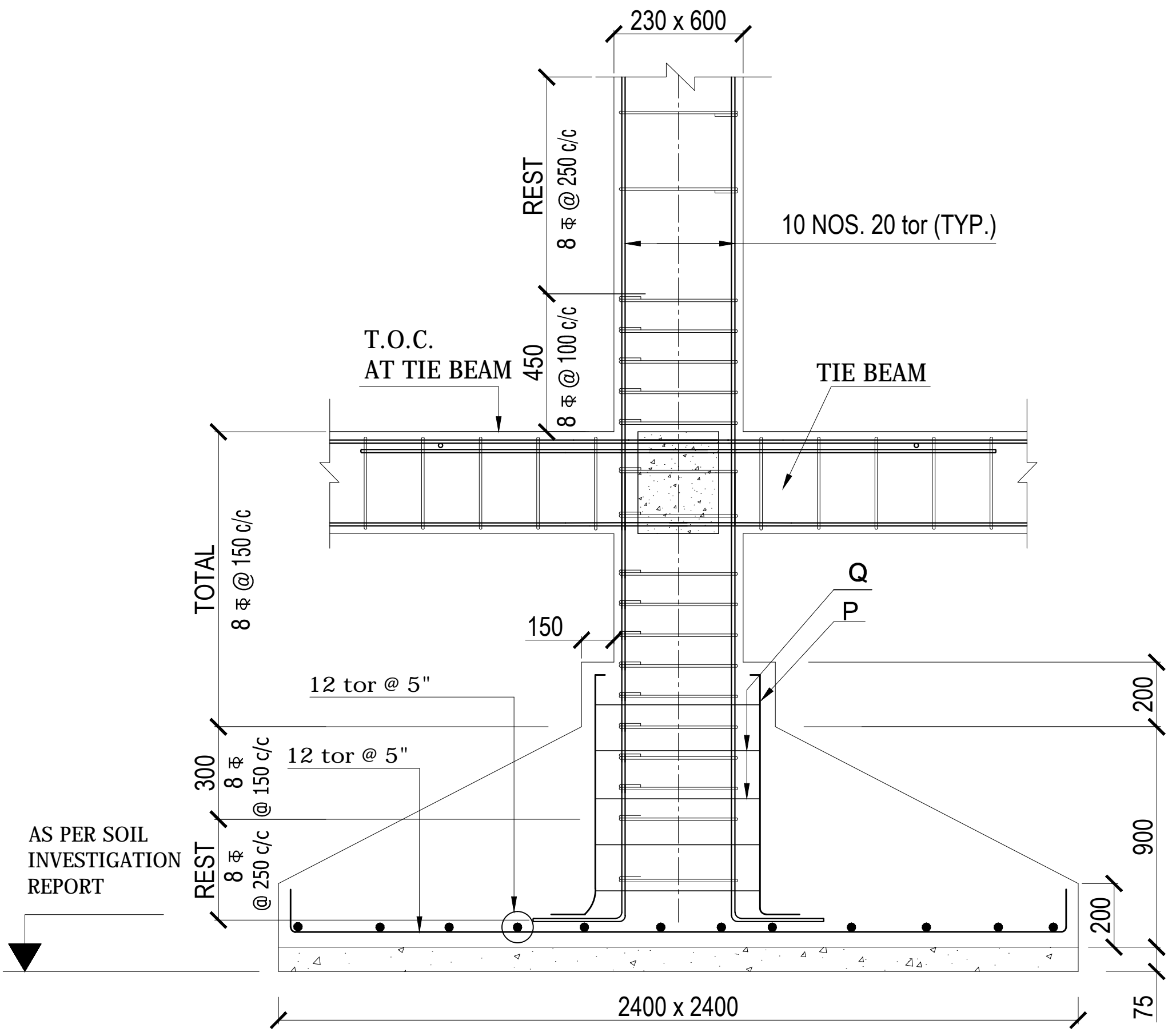
TYPICAL SECTION - COLUMN WITH FOUNDATION
