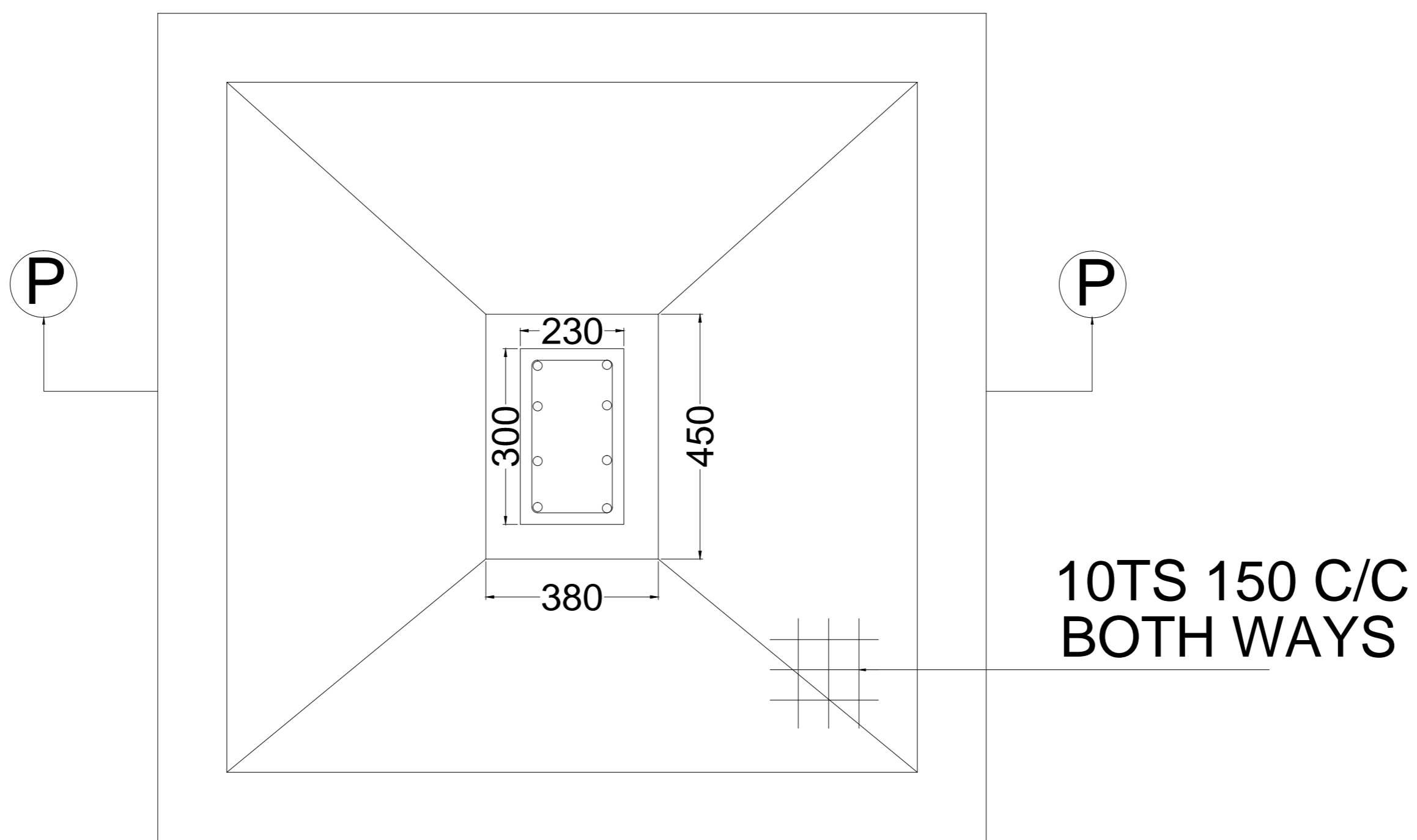
PLAN FOOTING PLAN (AS/STRL. DESIGN) SCALE N.T.S
